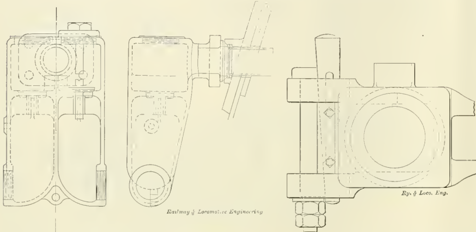
DOUBLE TOP CHECK ON BACK SHEET 4-4-2 PENNSYLVANIA LINES.
